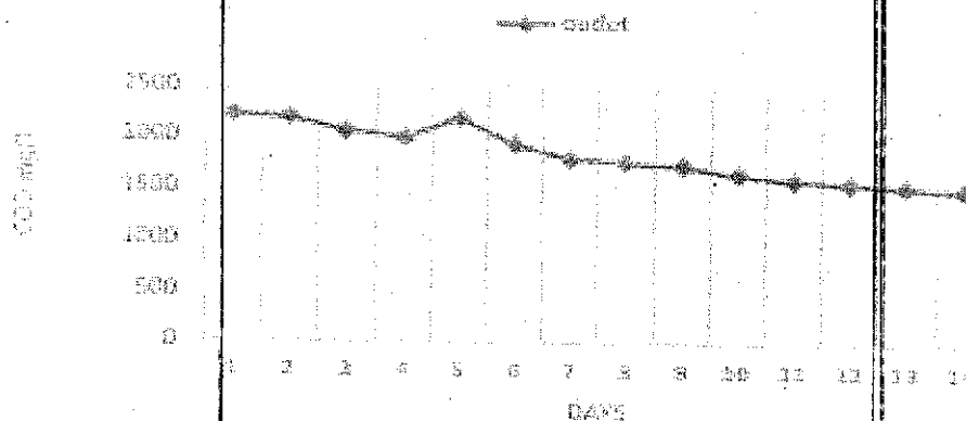
Chart 1.13: COD Removal at Inlet when DR- 1/1
