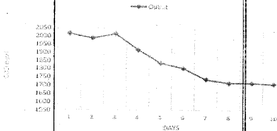
Chart 1.6: COD Removal at Outlet when DR- 1/6
