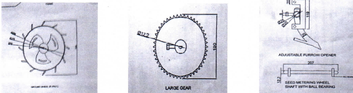
Fig. 3.4 An isometric view of drive wheel, large sprocket, adjustable furrow opener and seed metering device shaft of manually operated planter. (All dimensions in millimeter)
