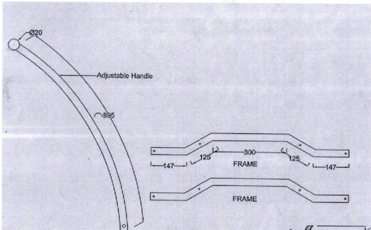
Fig. 3.1 An isometric view of adjustable handle and frame of manually operated planter. (All dimensions in millimeter)
