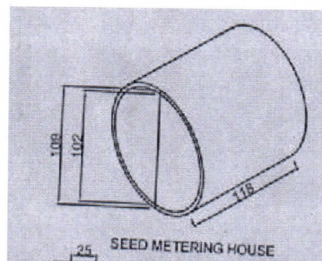
Fig. 3.3 An isometric view of seed metering device and seed metering house of manually operated planter. (All dimensions in millimeter)
